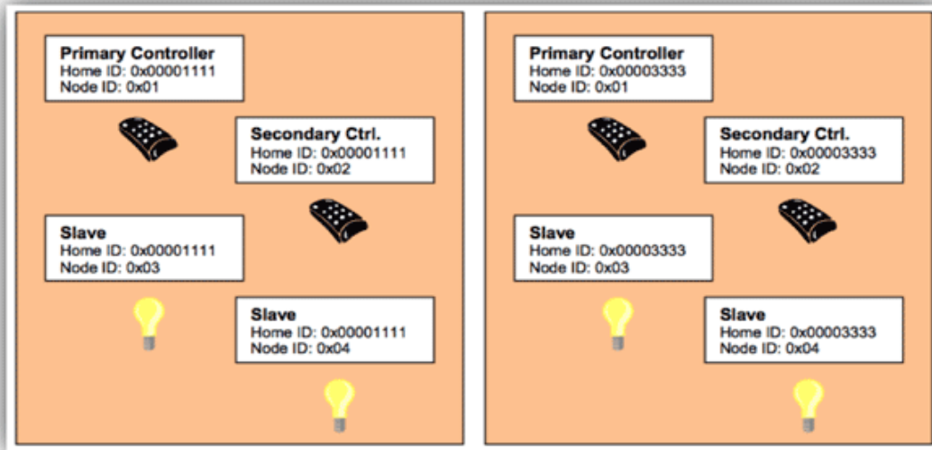
Two Z-Wave networks with different Home IDs co-exist
