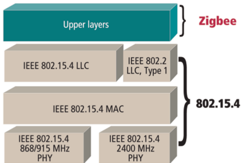
IEEE 802.15.4 RF CHANNEL DETAILS
